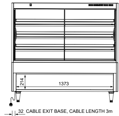
REAR ELEVATION
